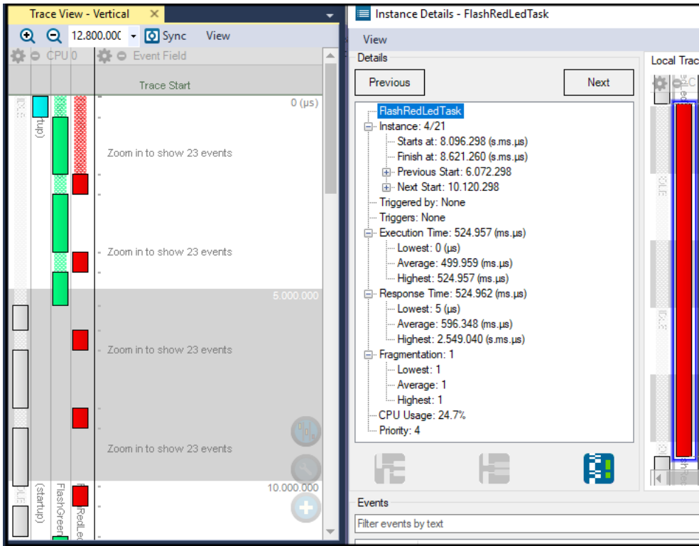
Figure 6.21 Trace recording - FlashRedLedTask and actor information
